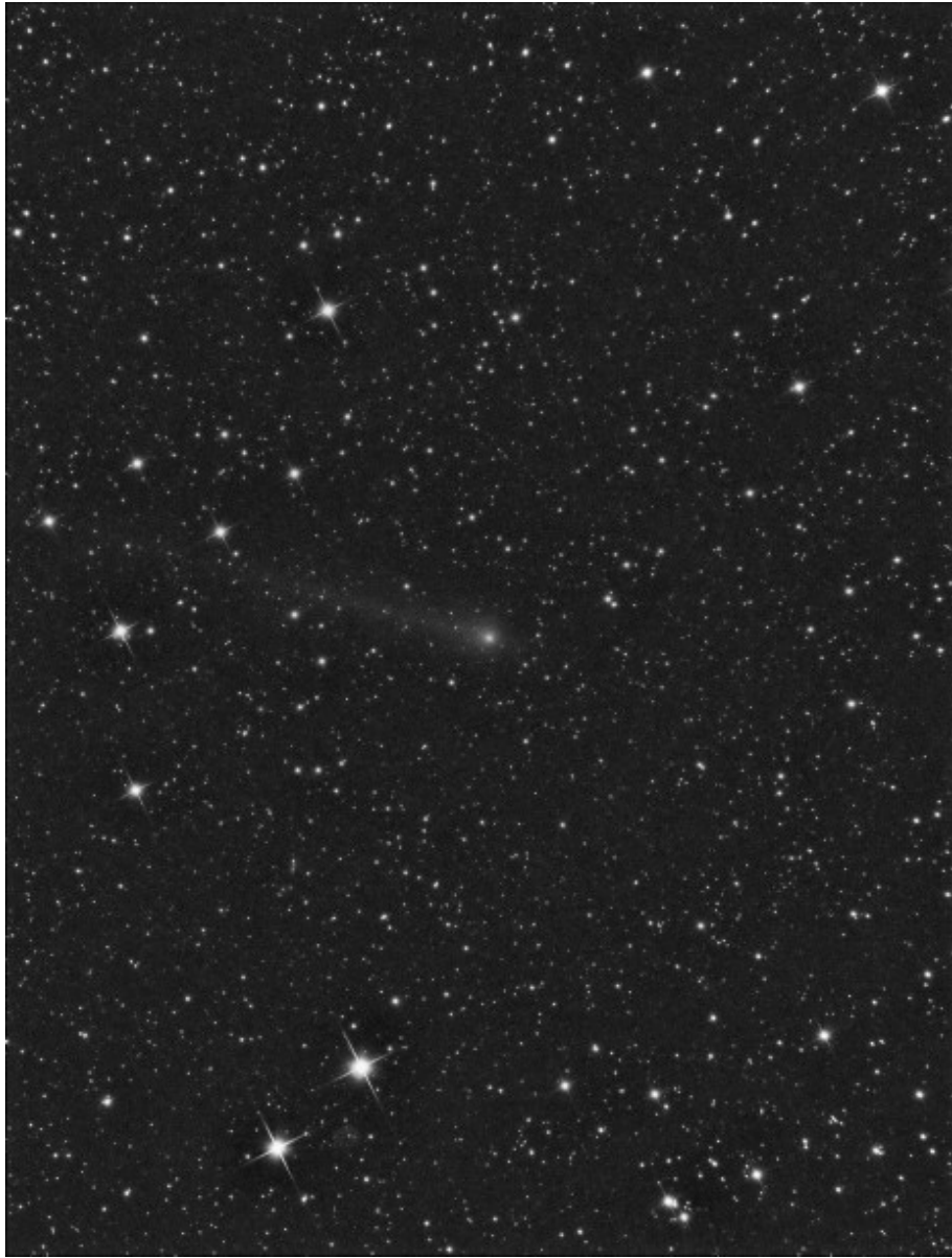
C/2012 F6 (LEMMON) - 02/09/2013
